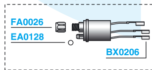
AR0005 2 spring pins 1 female pin
